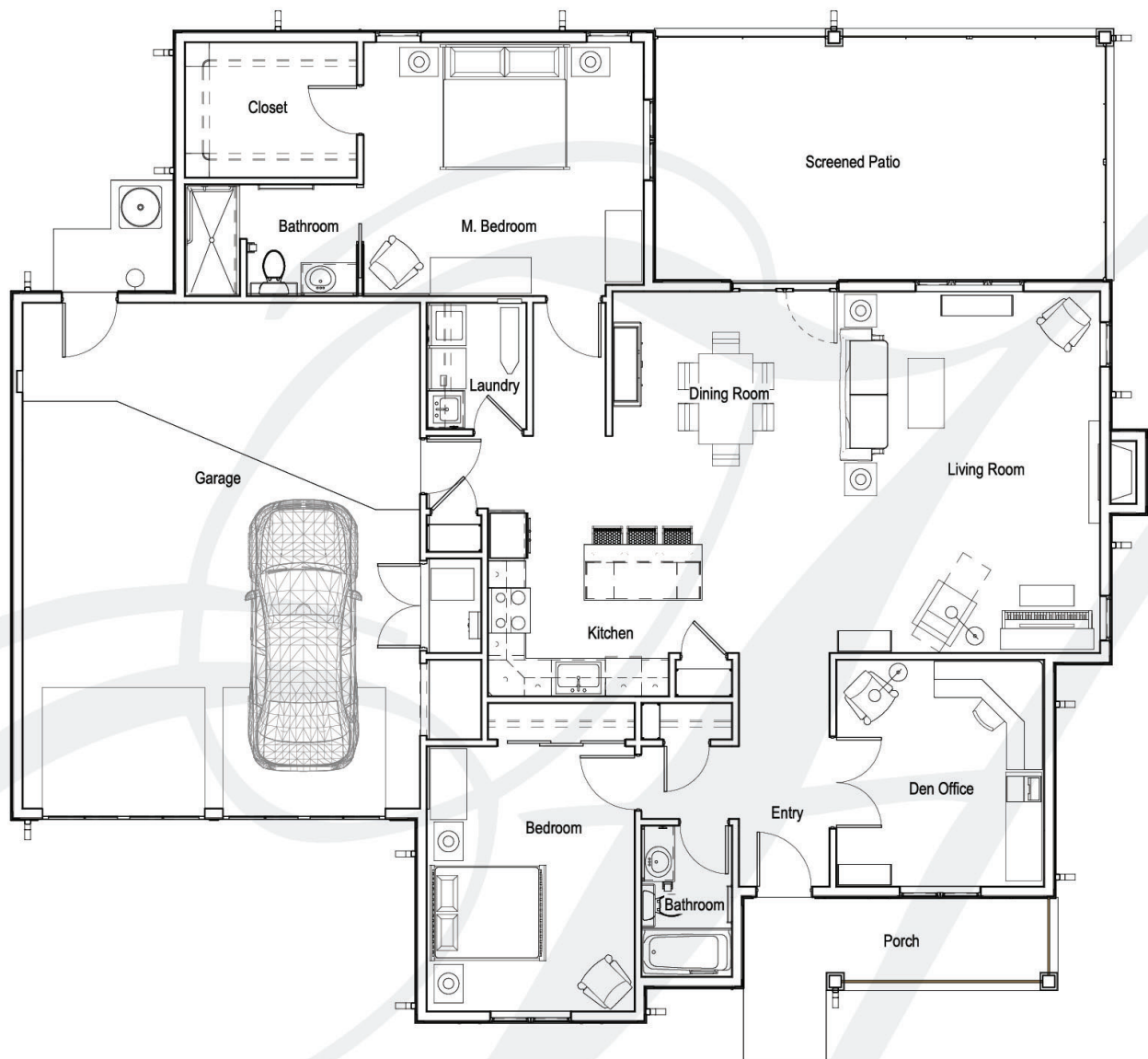
VILLA III Two Bedroom - 1700 Sq. Ft.
