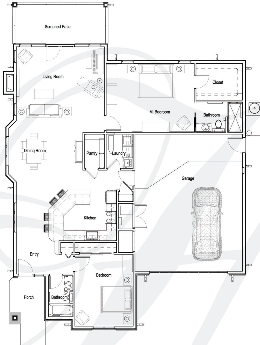
VILLA II Two Bedroom - 1650 Sq. Ft.
